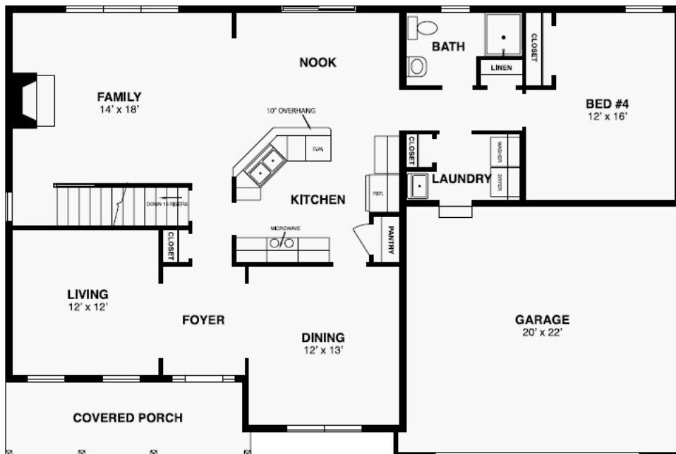
1st Floor
